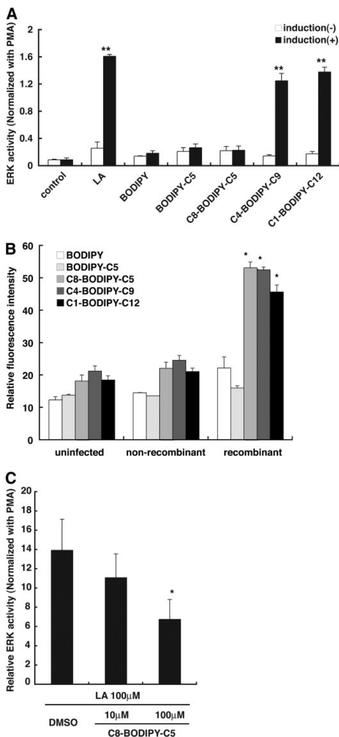
Fig. 3. Effects of BODIPY-FFAs on GPR40. A , effects of BODIPY-FFAs on ERK-1/2 activation in T-Rex hGPR40 cells. T-Rex hGPR40 cells that had been incubated with Dox [■, induction (+)] or without Dox [□, induction (-)] for 24 h were stimulated with each compound at a concentration of 100 \mu M. Cell lysates were analyzed by immunoblotting using anti-phospho- and anti-total-kinase antibodies. The amount of phosphorylated ERK-1/2 was normalized to the amount of total ERK-1/2. Then the data were expressed as -fold difference relative to the amount of ERK-1/2 phosphorylation that was obtained in the presence of phorbol 12-myristate 13-acetate (PMA). Results are means \pm S.E. of three independent experiments. Significant differences (*, p < 0.05 ; **, p < 0.01 ) between treatment with the control (DMSO only) and with the compound. B , interaction of BODIPY-FFAs with solubilized GPR40 protein that had been immobilized on the beads. BODIPY-FFAs (3 \mu M) were added to the
